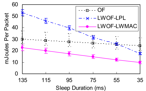
Fig. 8. Normalized energy consumption of different forwarding schemes for sensor networks with different duty cycles
