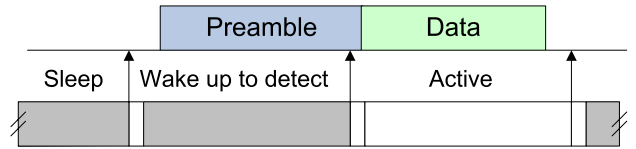
Fig. 1. Packet transmission with an LPL MAC protocol (B-MAC)
